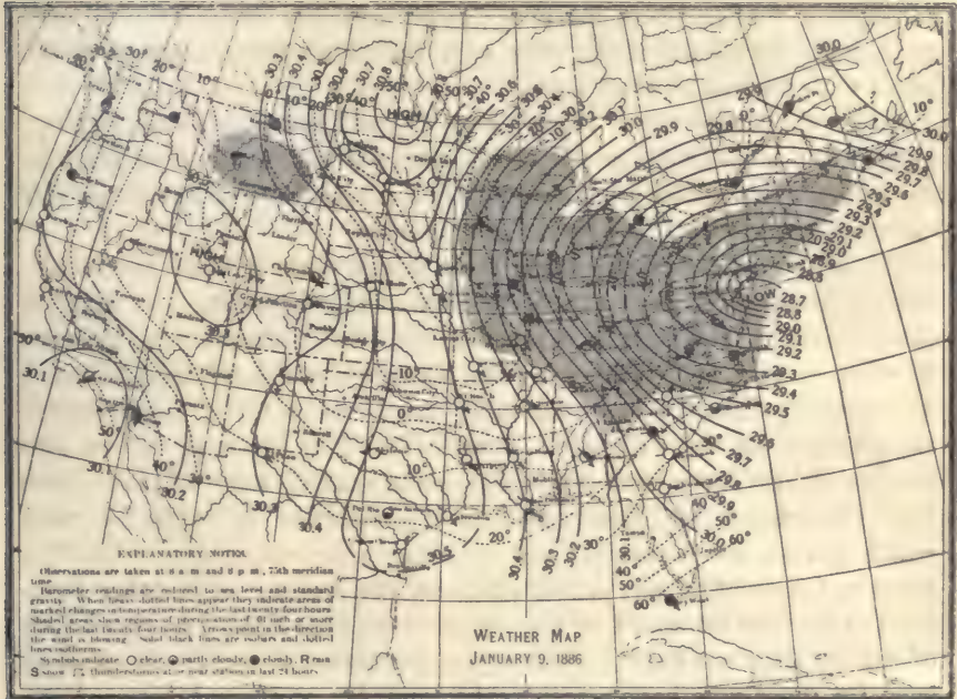
FIGURE 67. Weather Map of January 9, 1886.
